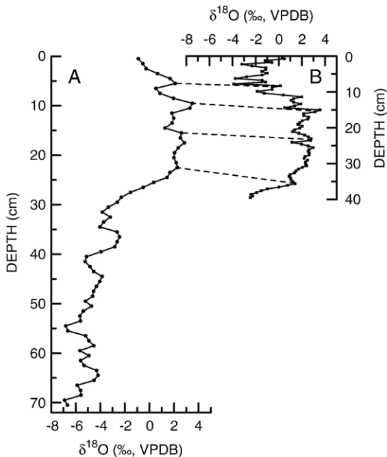
Fig. 3. Correlation of the \delta^{18}O records from core WLC002 (A) and WLB003C (B). Dashed lines indicate the suggested tie points between the two records.
